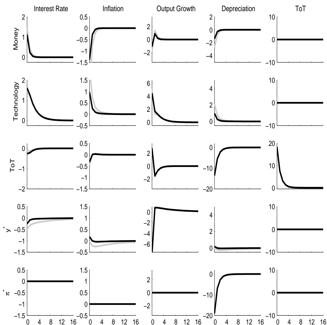
Figure 6: DSGE MODEL IMPULSE RESPONSES AS FUNCTION OF \psi_1
