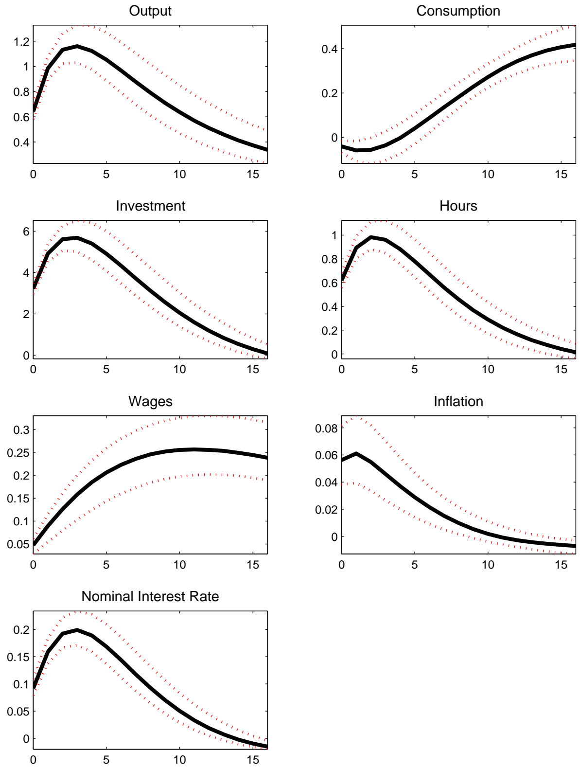
Figure 2: Impulse response to a MEI shock
