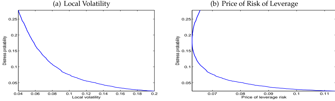
Figure 7. Volatility Paradox
